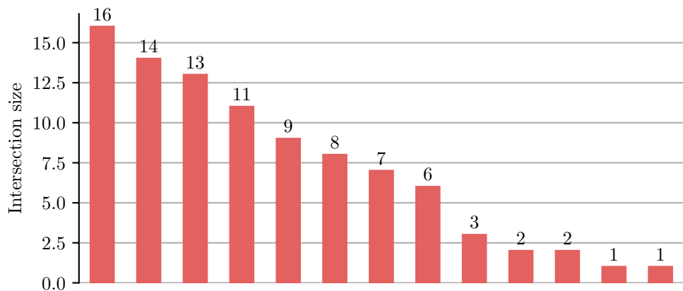
Shrinkage Intersections (pass@256 Base=1, RL=0), Model: Llama3.1-8B-Instruct
